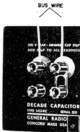
Figure 6. Type 1412-BC with two-terminal (grounded) connection using bus wire.
