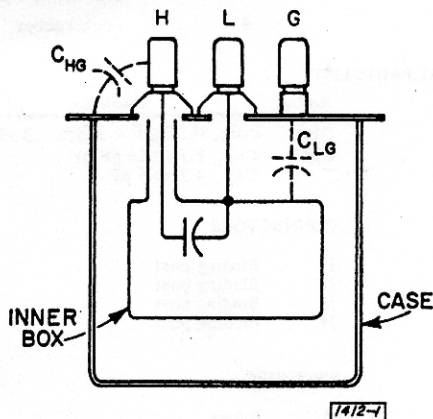
Figure 1. The double shielding used in the Type 1412-BC Decade Capacitor keeps CHG very small. This capacitance is the difference between the three-terminal and two-terminal capacitance of the box; CLG is approximately 125 pF.
